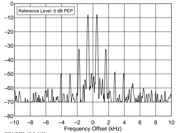
ICOM IC-706mKII G 01674 432.200 MHz, Transmit IMD, 20 W F:\SHARED\PROD_REV\TESTS\IC706G\IC706I70.TXT
